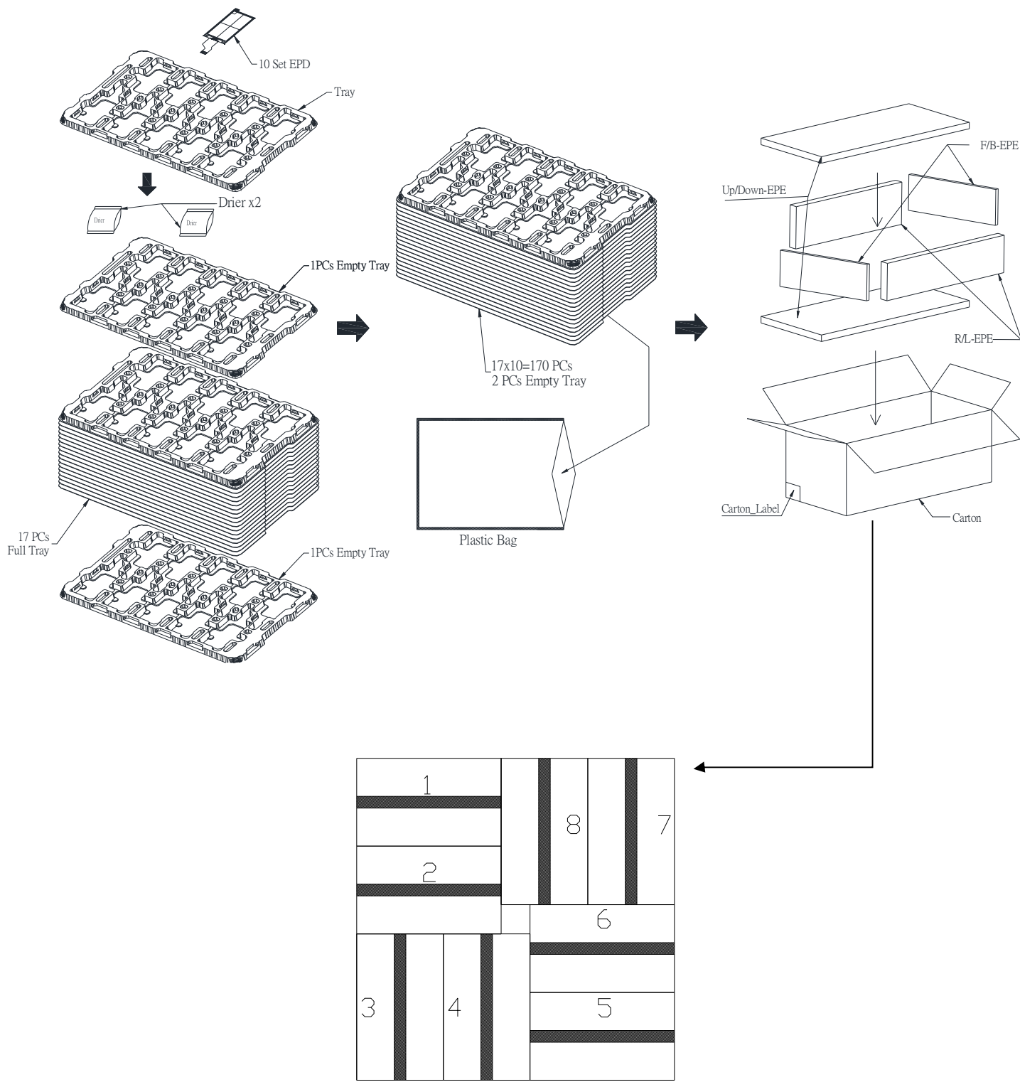
Figure 7-1 Packing Diagram
