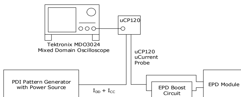
Figure 3-3 Current Measurement
