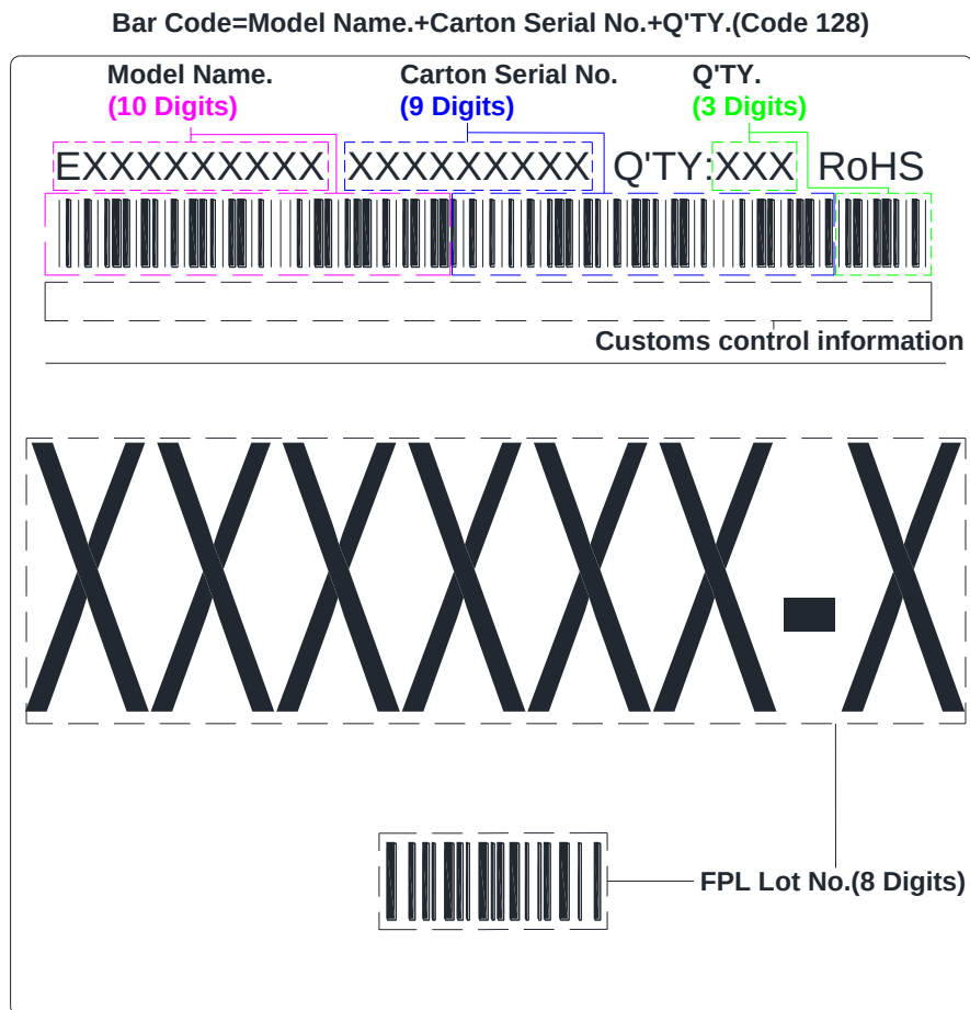
Figure 9-3 Carton Label
