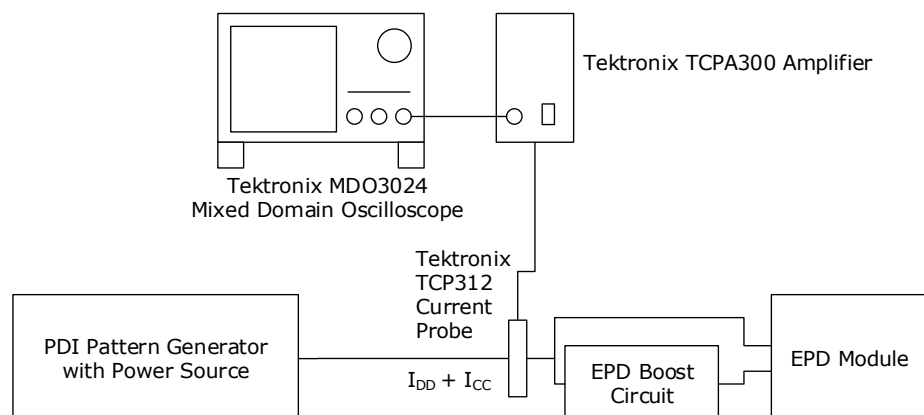
Figure 3-3 Current Measurement
