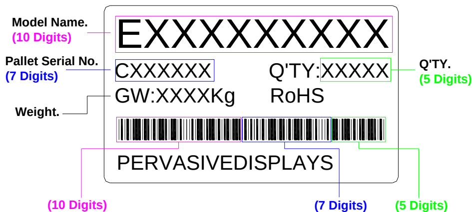
Figure 9-4 Pallet Label
