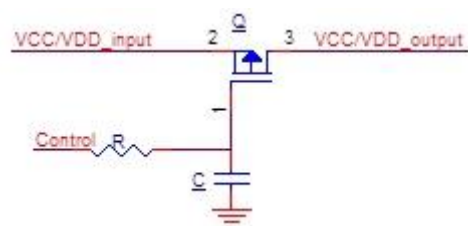
VCC/VDD soft-start
