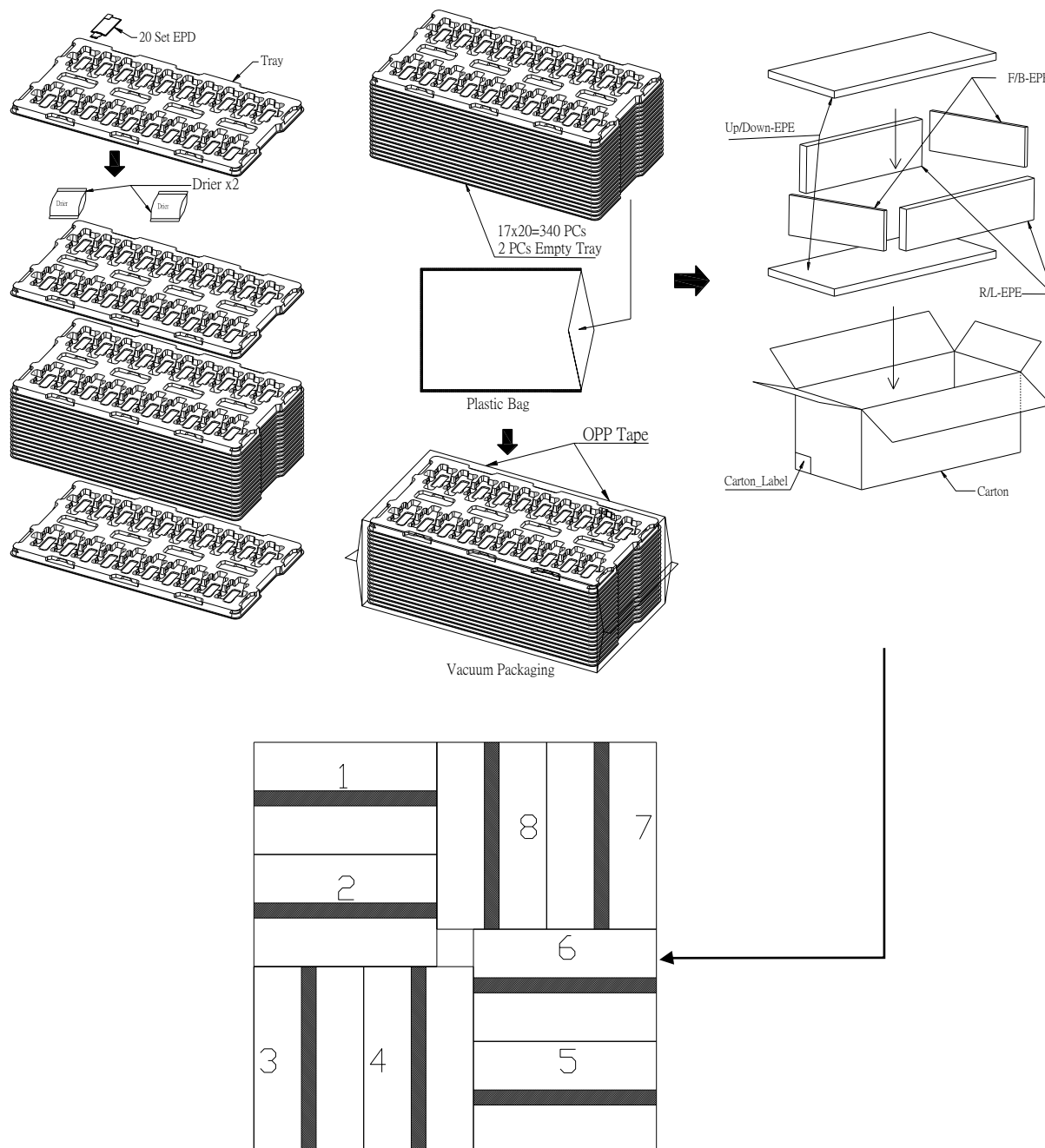
Figure 7-1 Packing Diagram
