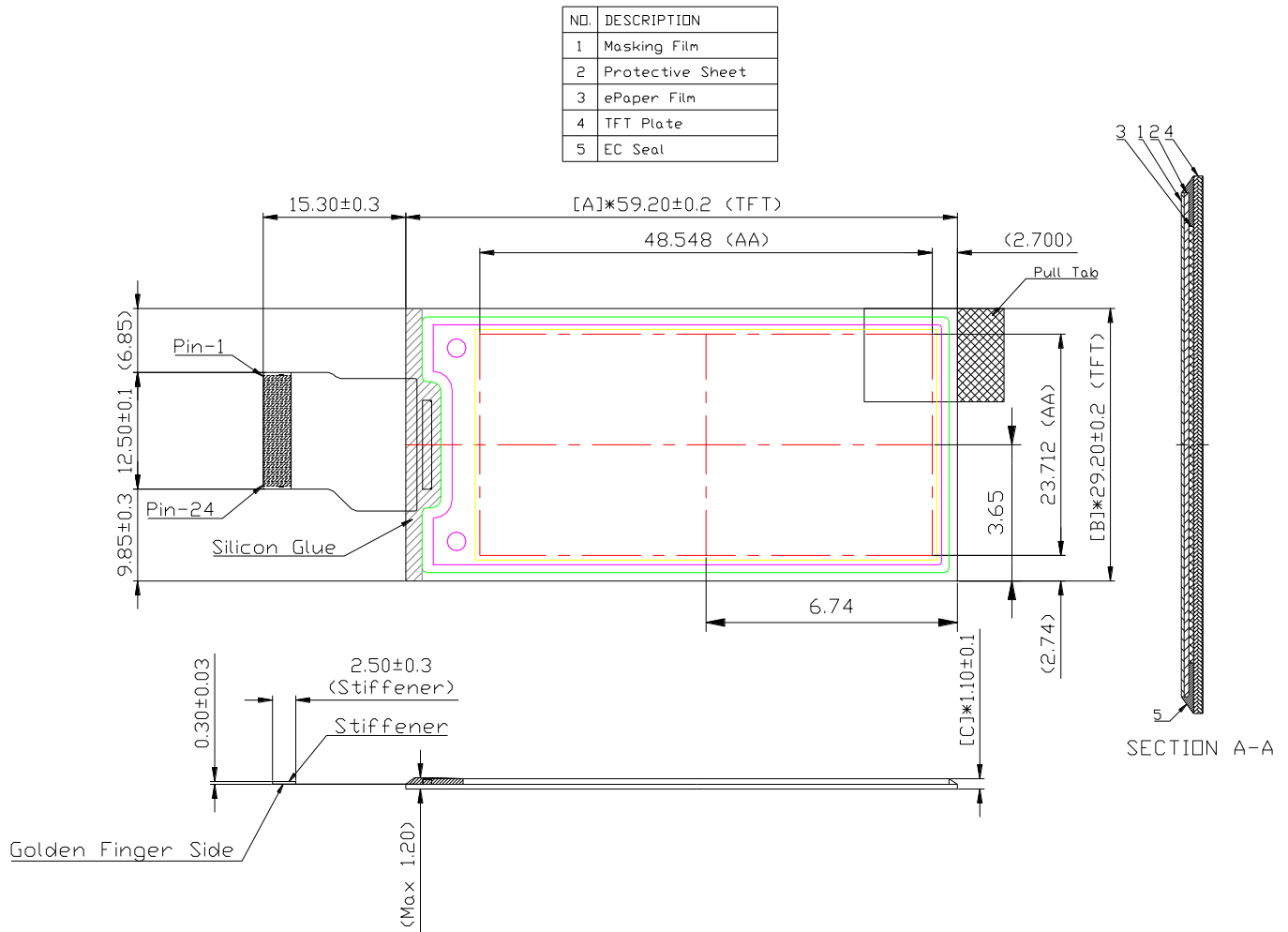
Figure 1-1 EPD Drawing
