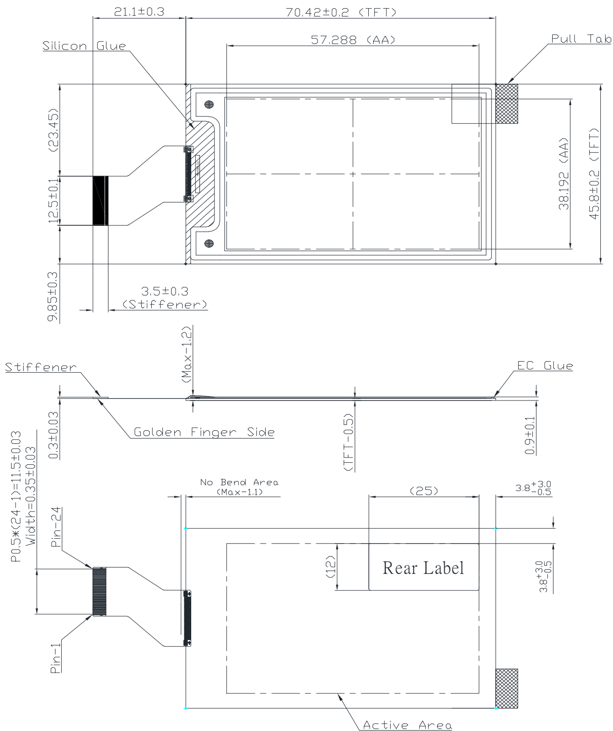
Figure 1-1 EPD Drawing
