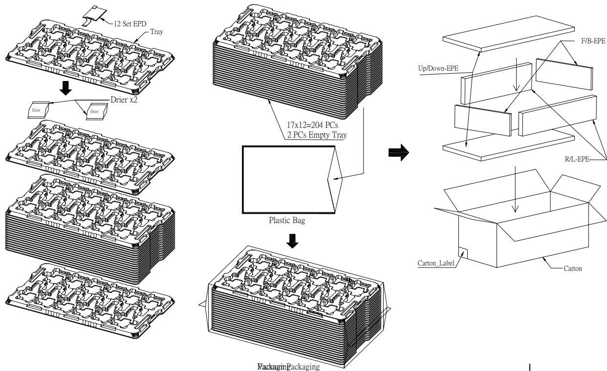
Figure 7-1 Packing Diagram
