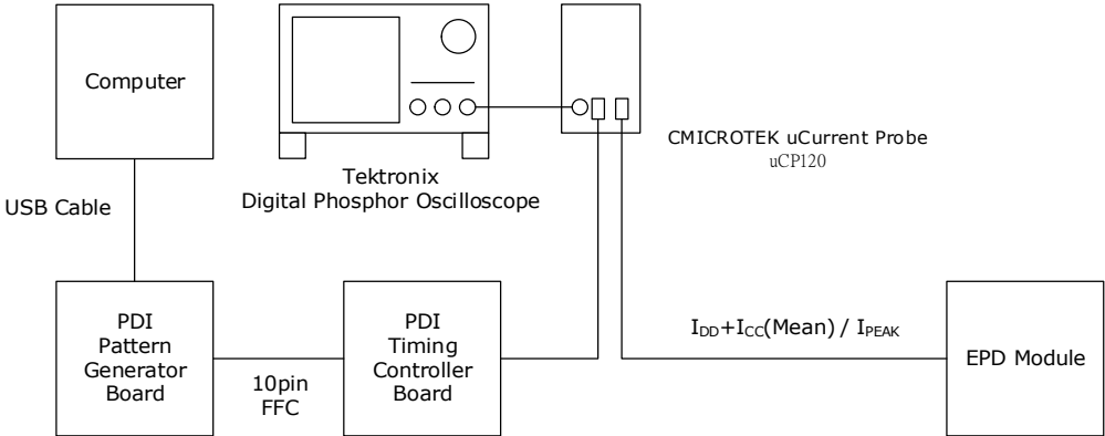
Figure 3-3 Current Measurement
