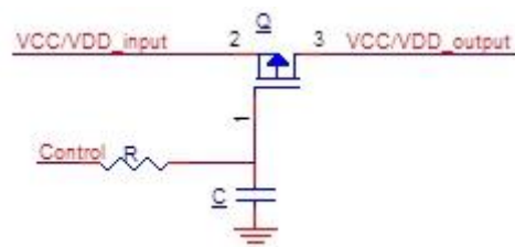
VCC/VDD soft-start
