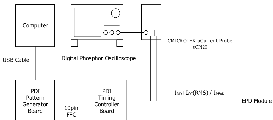
Figure 3-3 Current Measurement
