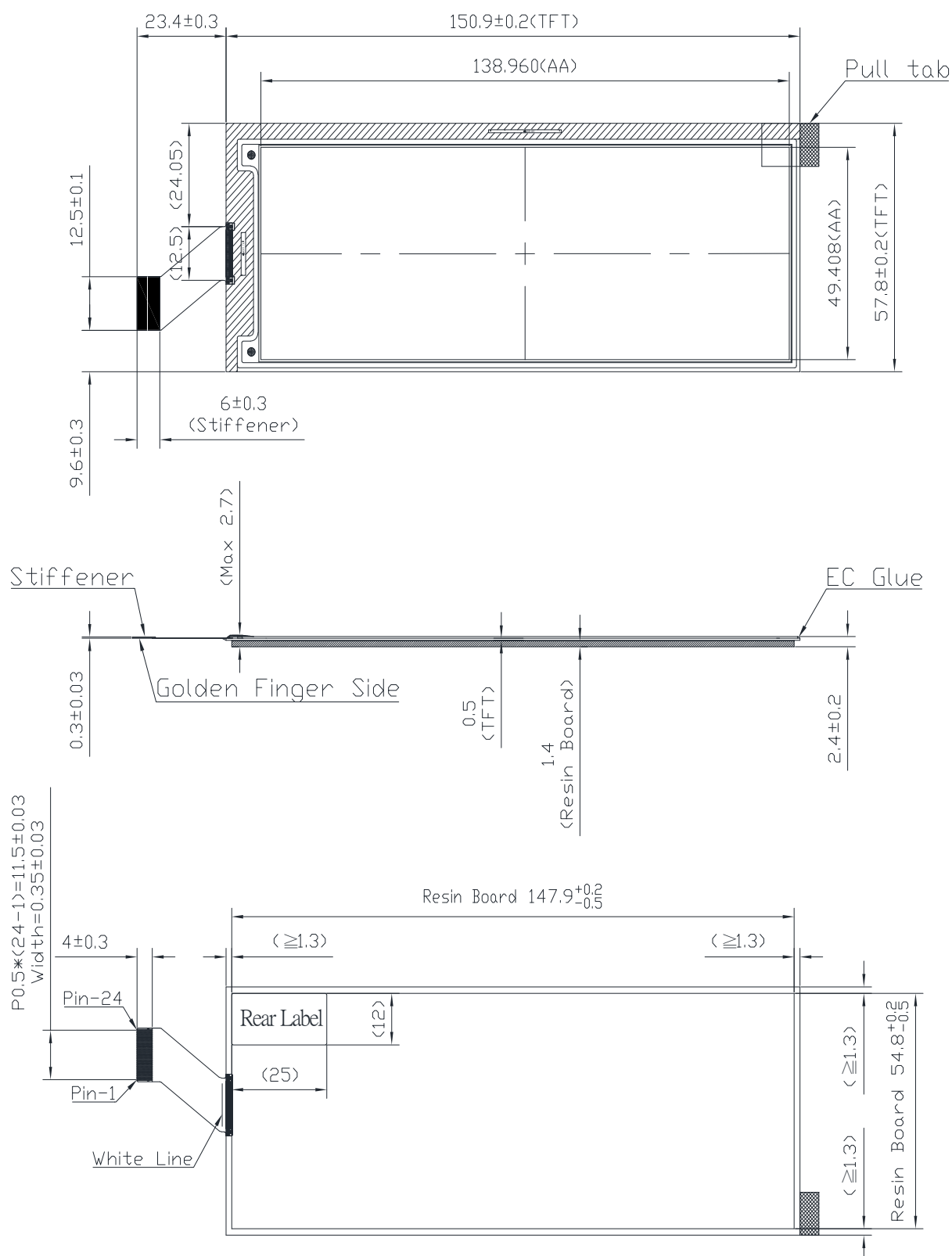
Figure 1-1 EPD Drawing
