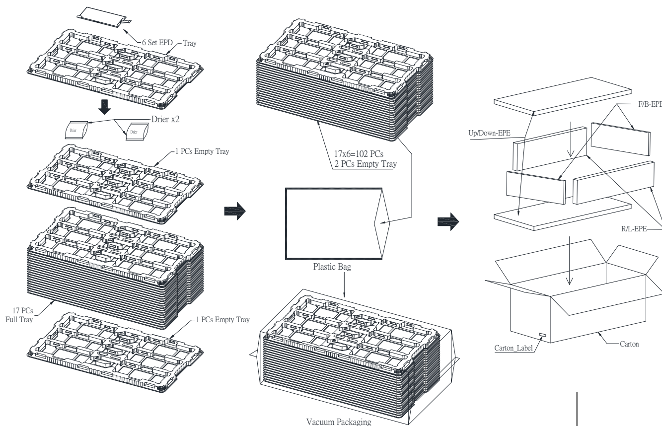
Figure 7-1 Packing Diagram
