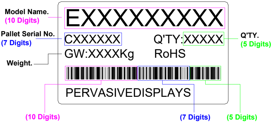
Figure 9-3 Pallet Label
