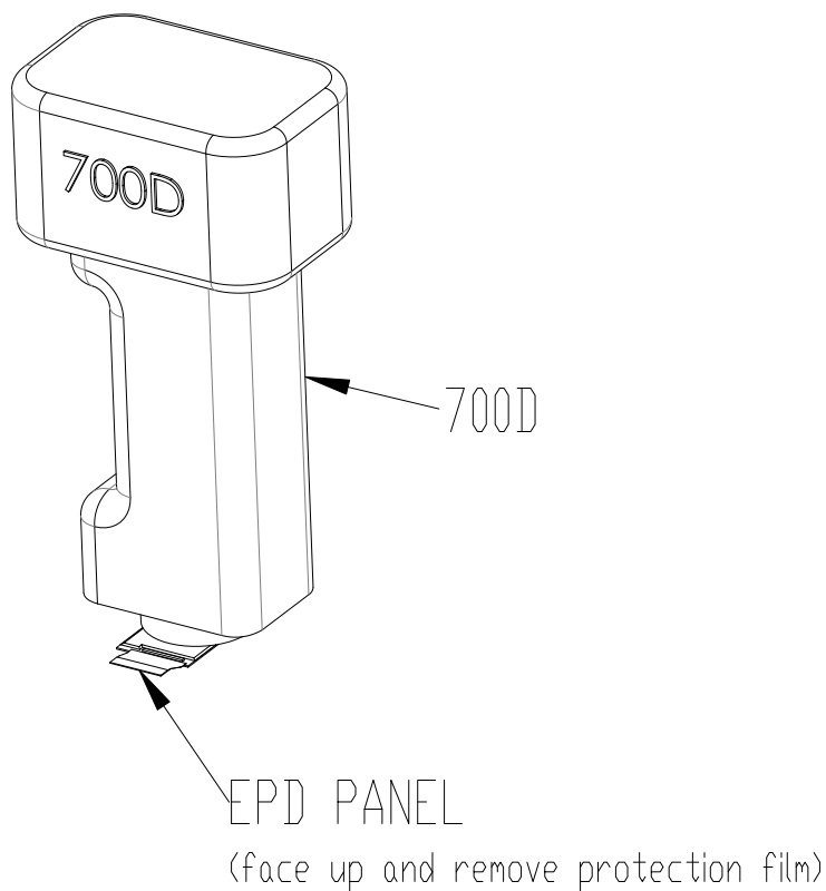
Figure 6-1 Optical measurement
