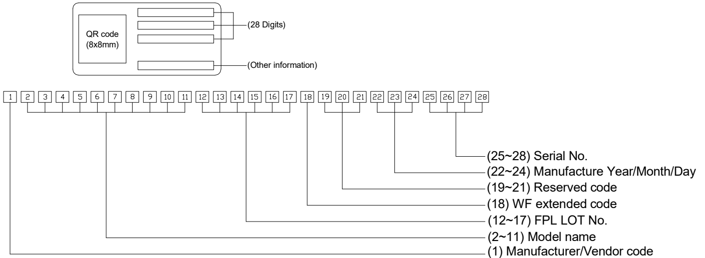
Figure 9-2 Carton Label
