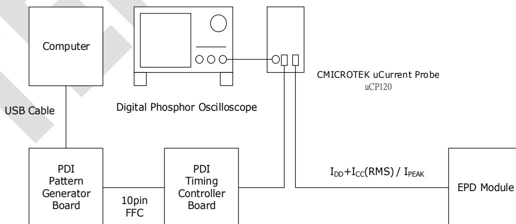
Figure 3-3 Current Measurement
