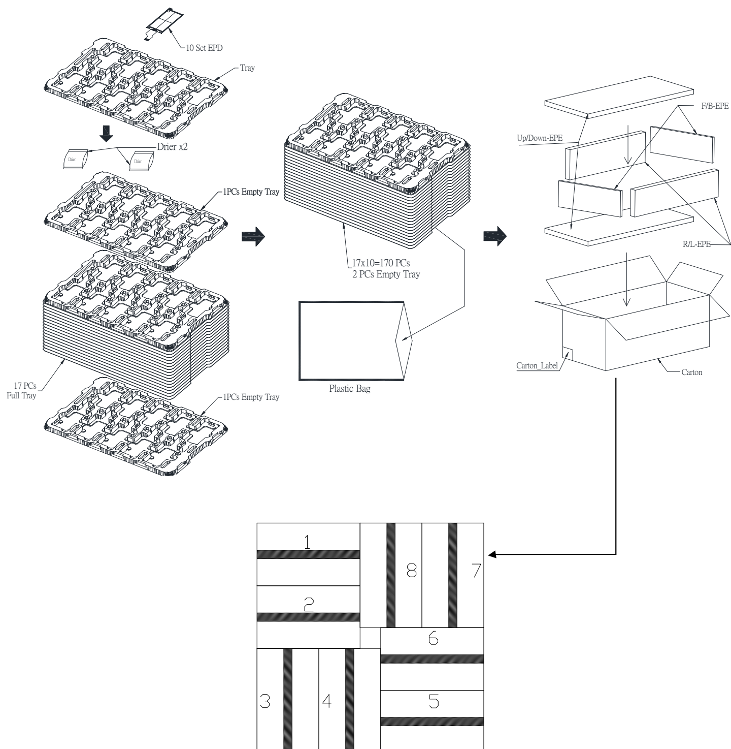
Figure 7-1 Packing Diagram
