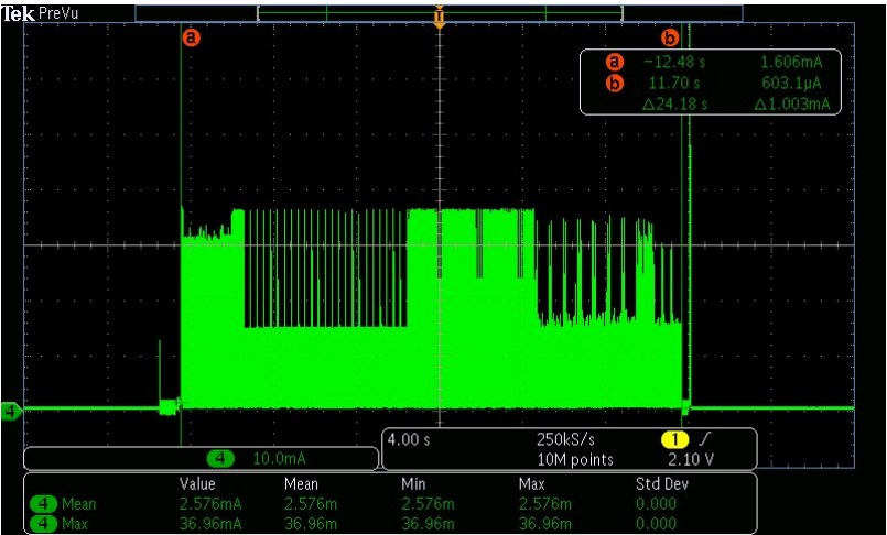
Figure 3-2 Image Update Current Profile
