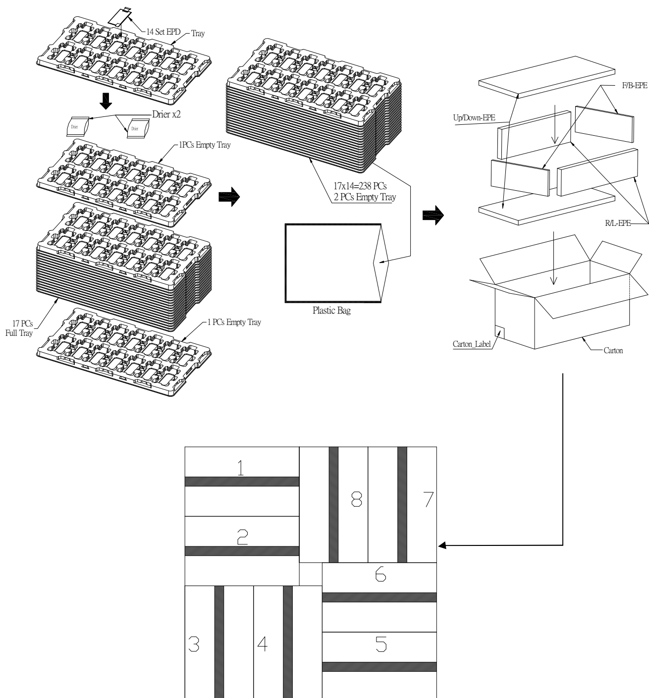
Figure 7-1 Packing Diagram
