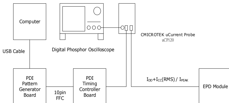
Figure 3-3 Current Measurement
