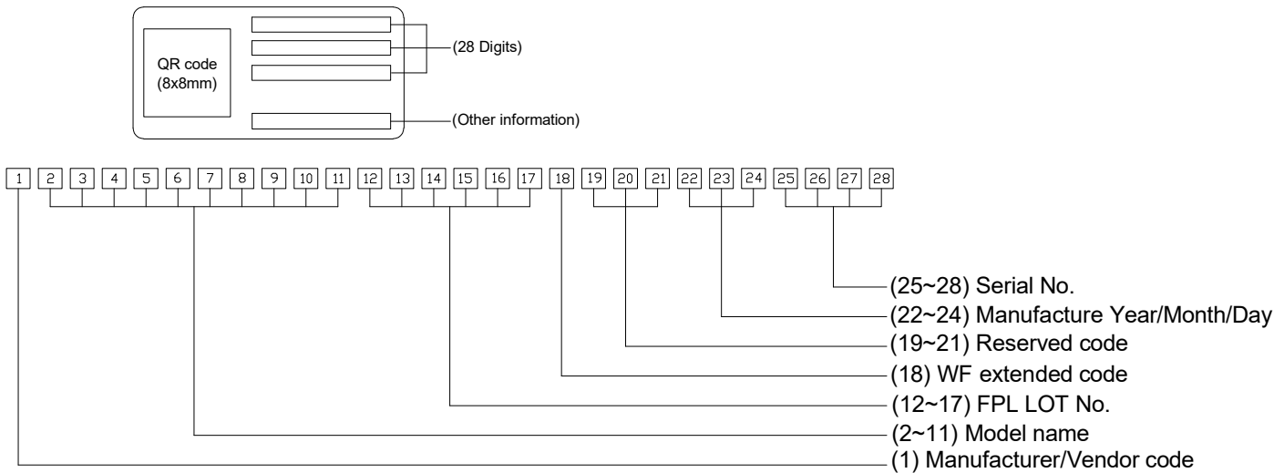
Figure 9-2 Carton Label
