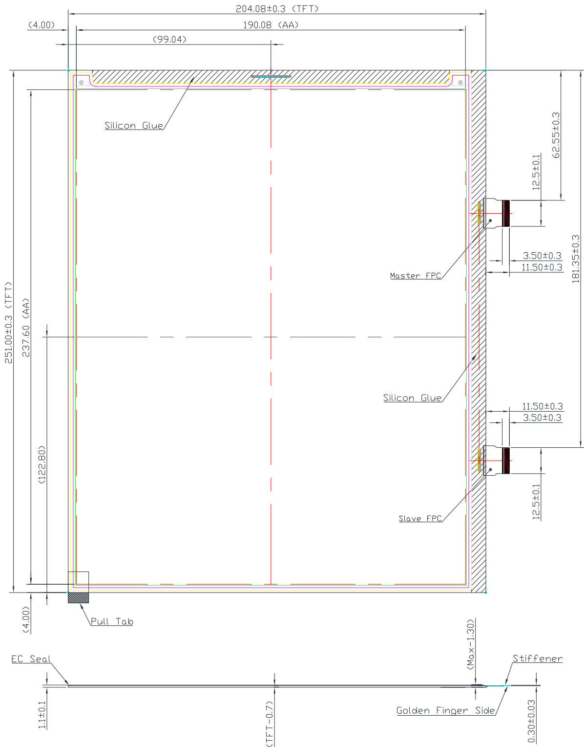
Figure 1-1 EPD Drawing
