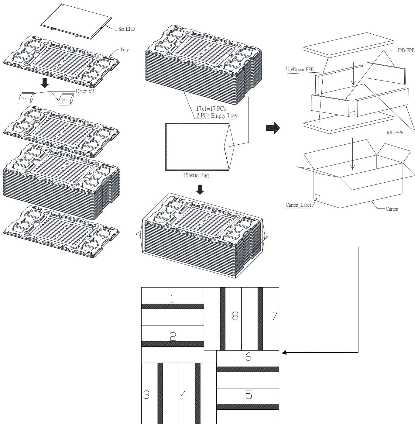
Figure 7-1 Packing Diagram
