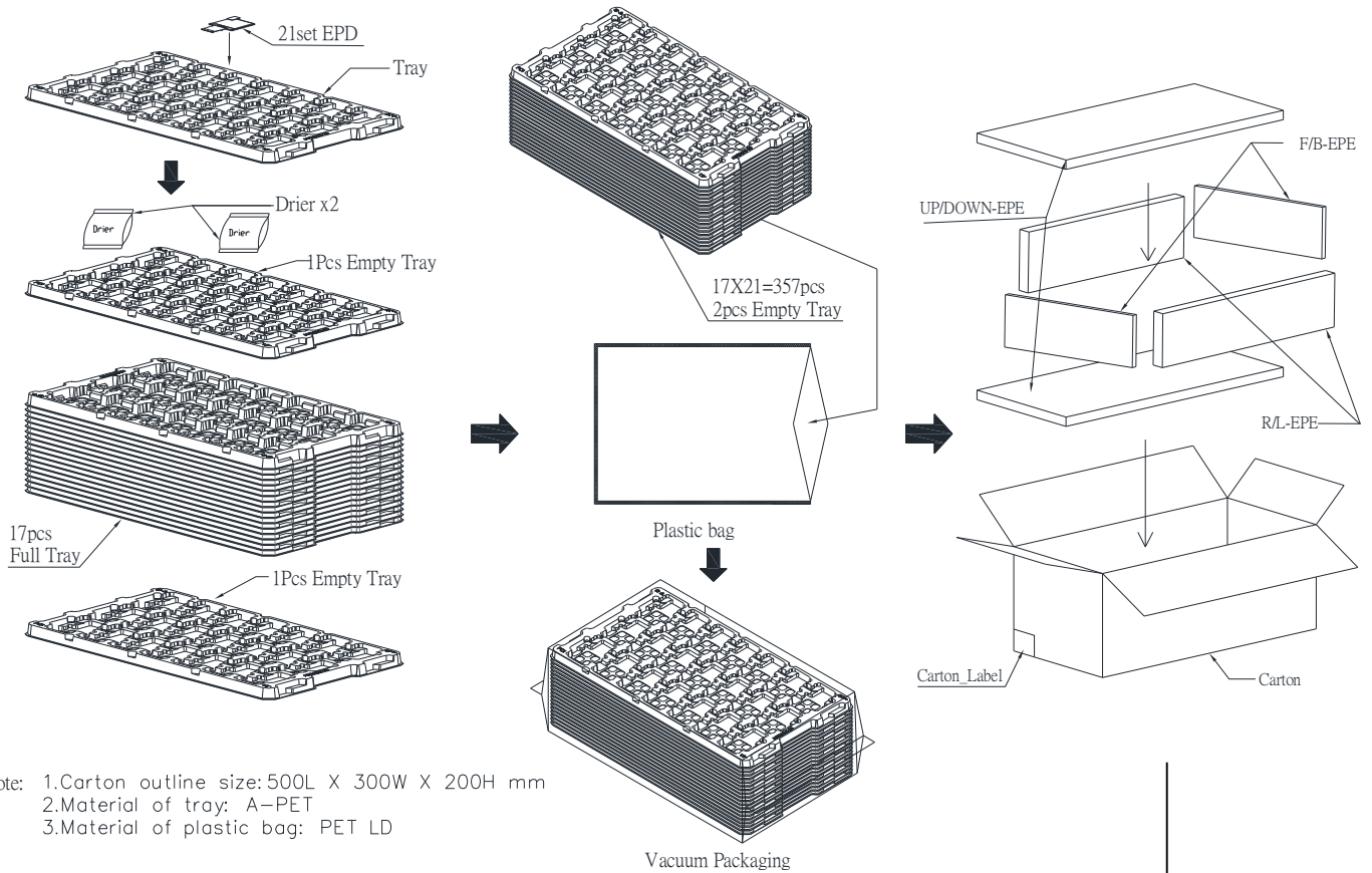
Figure 7-1 Packing Diagram
