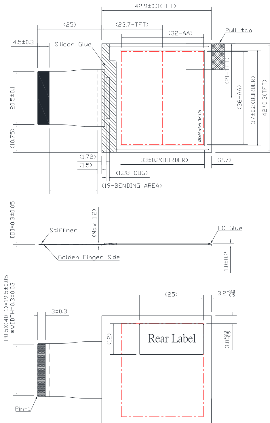
Figure 1-1 EPD Drawing
