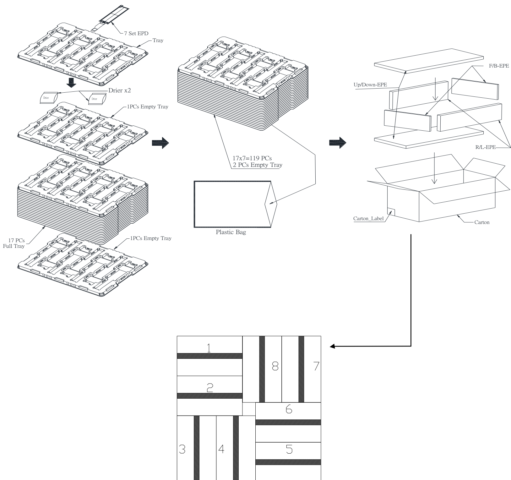
Figure 7-1 Packing Diagram
