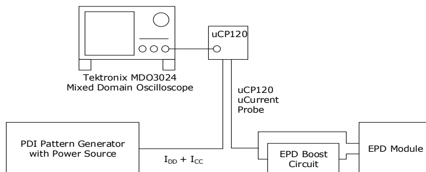
Figure 3-3 Current Measurement
