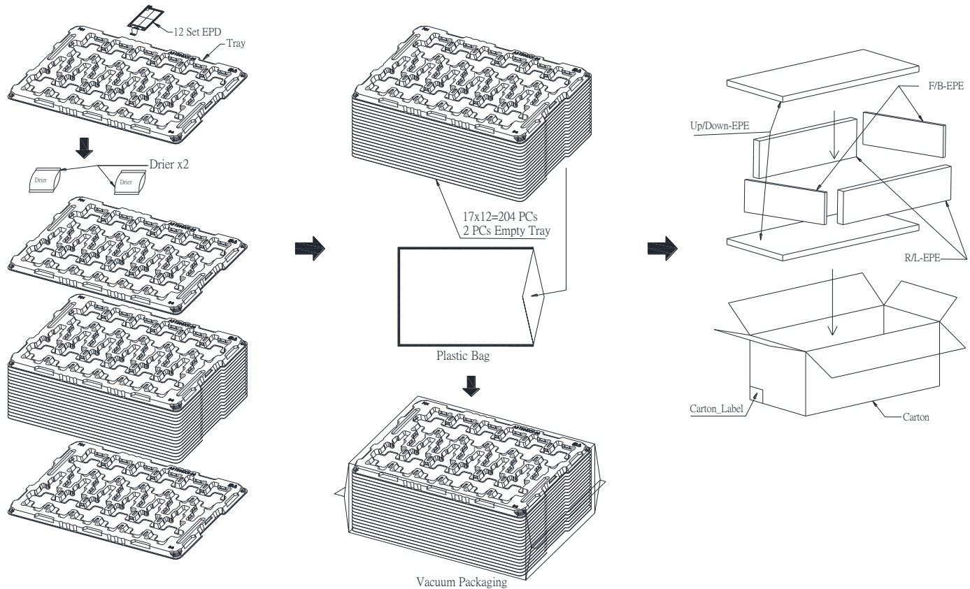
Figure 7-1 Packing Diagram
