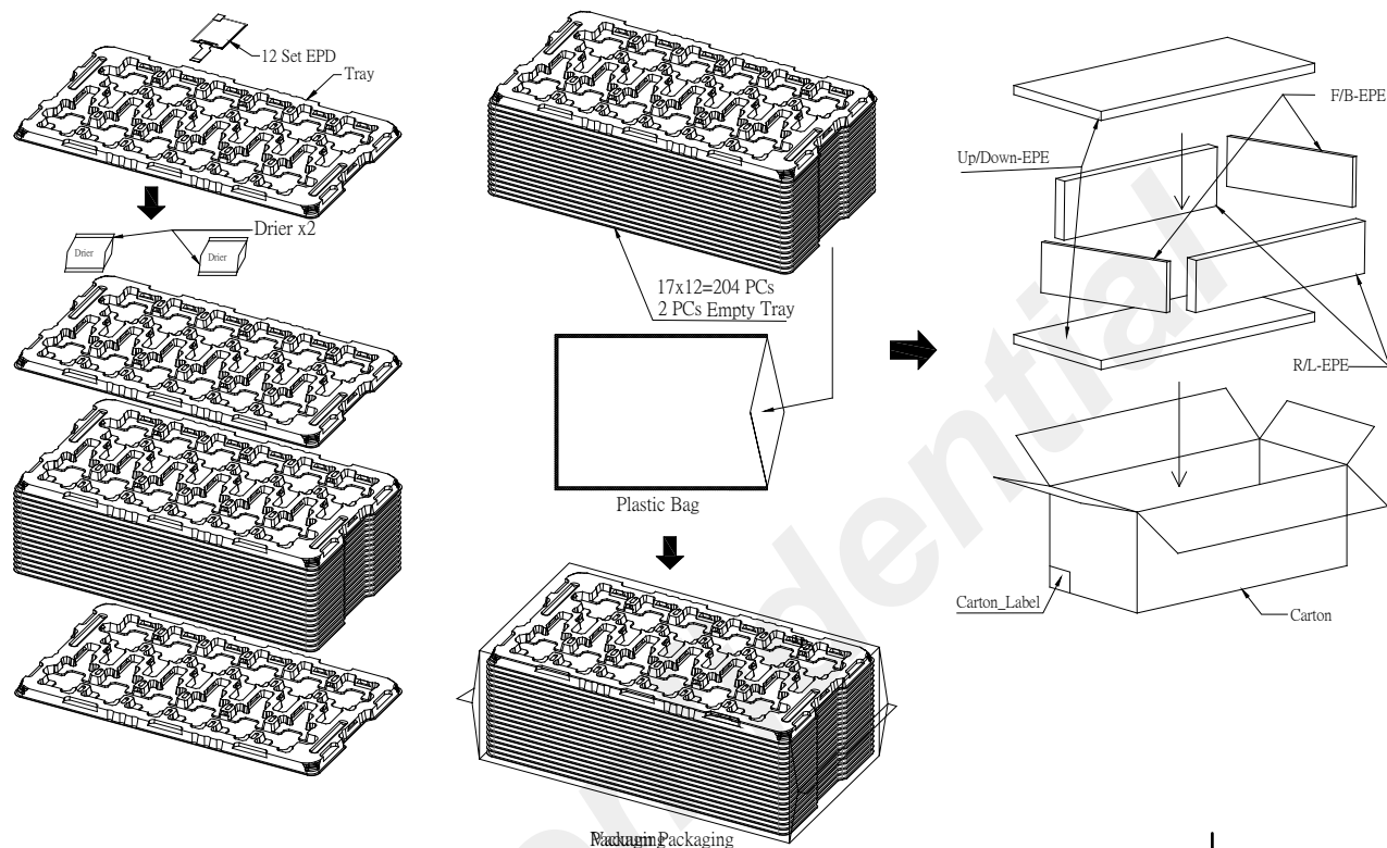
Figure 7-1 Packing Diagram
