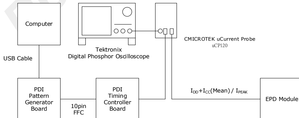
Figure 3-3 Current Measurement
