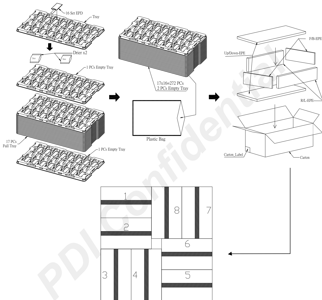
Figure 7-1 Packing Diagram
