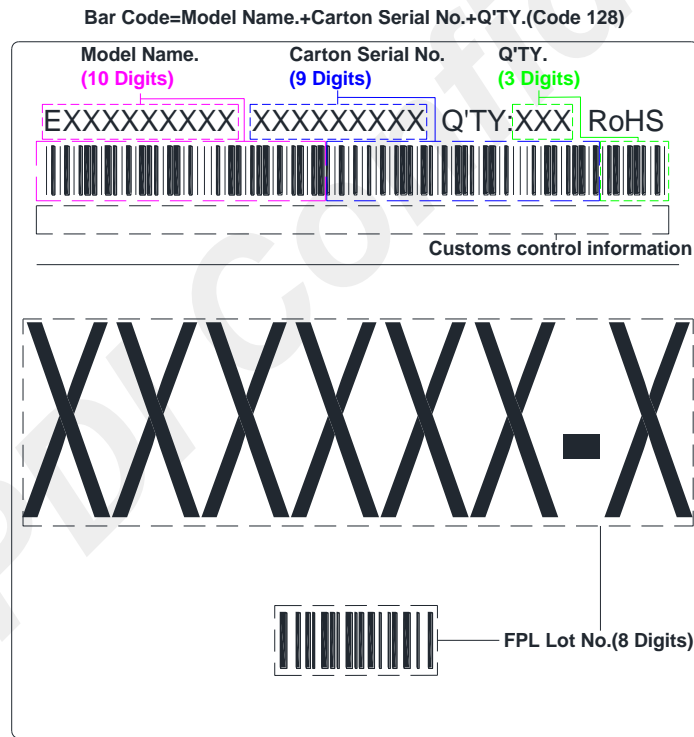
Figure 9-2 Carton Label
