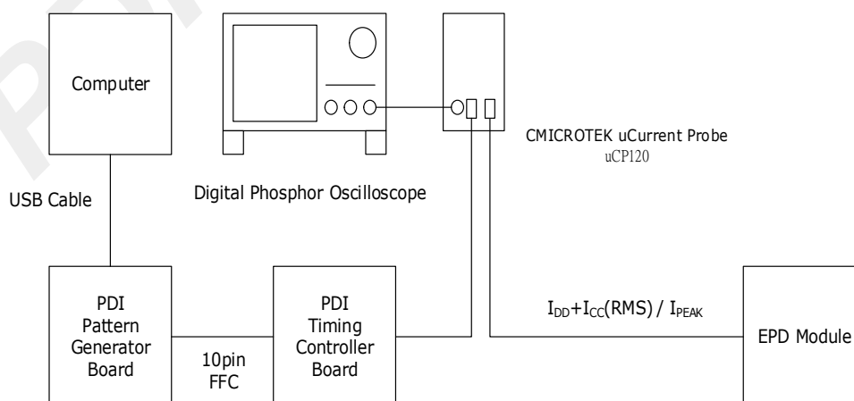
Figure 3-3 Current Measurement
