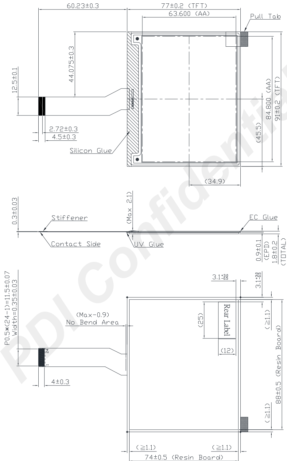
Figure 1-1 EPD Drawing
