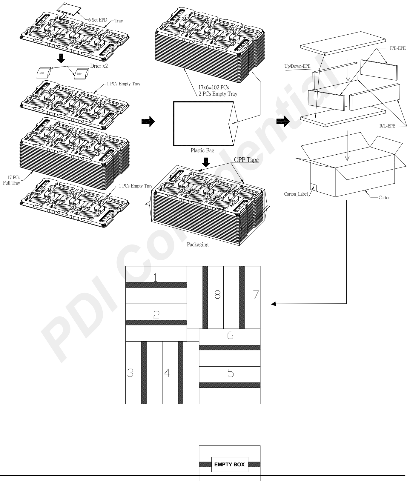
Figure 7-1 Packing Diagram
