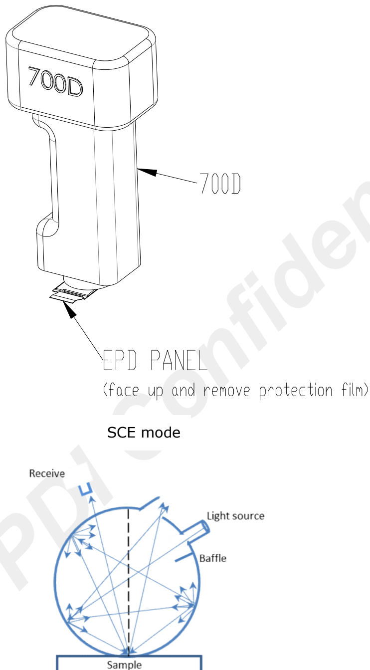
Figure 6-1 Optical measurement
