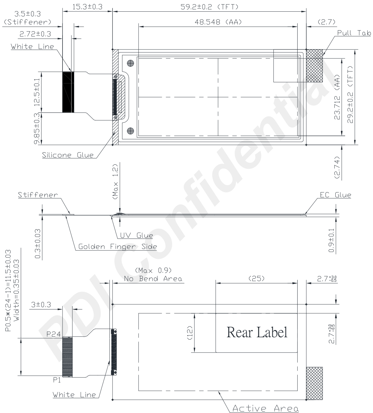
Figure 1-1 EPD Drawing
