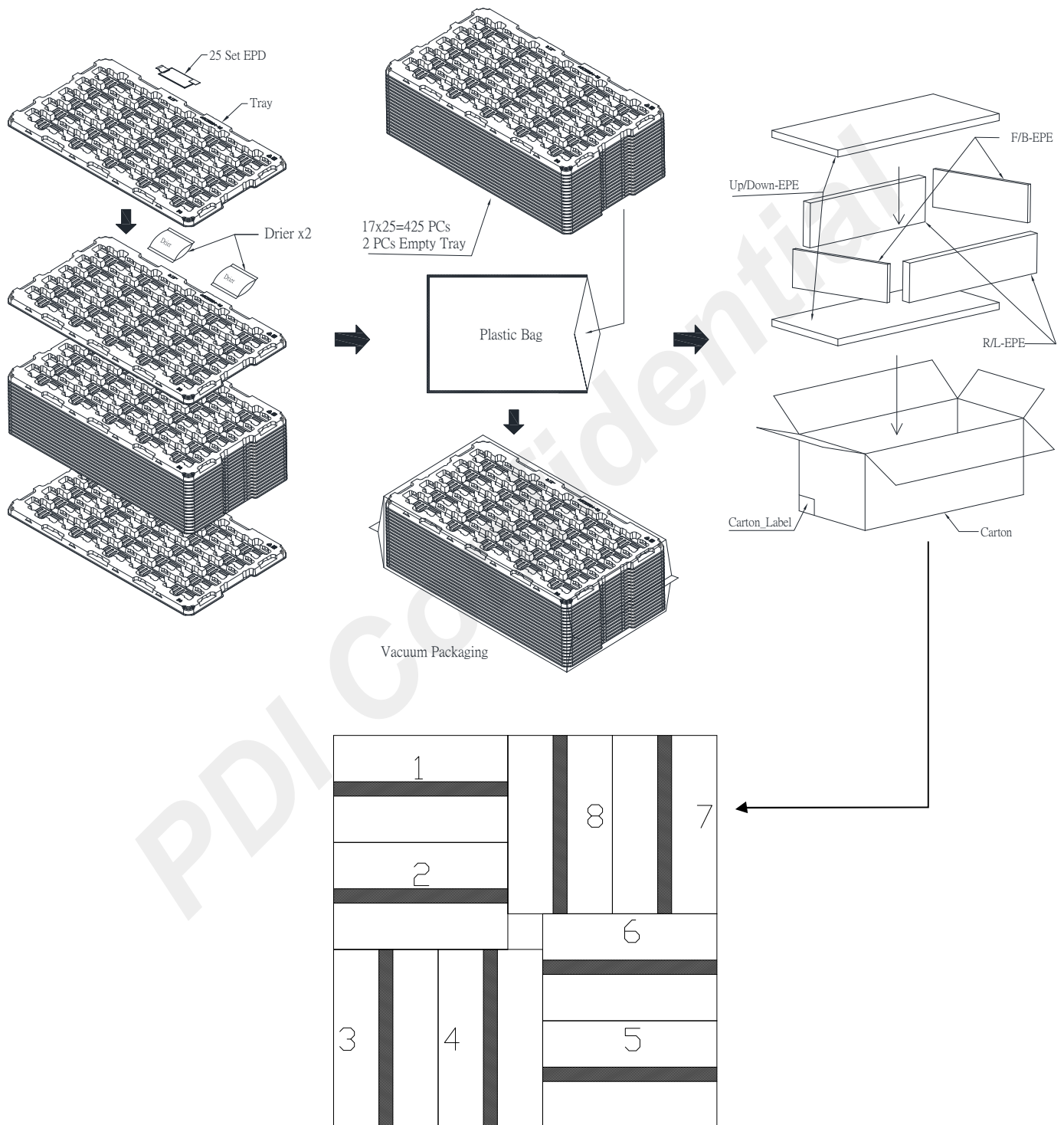
Figure 7-1 Packing Diagram
