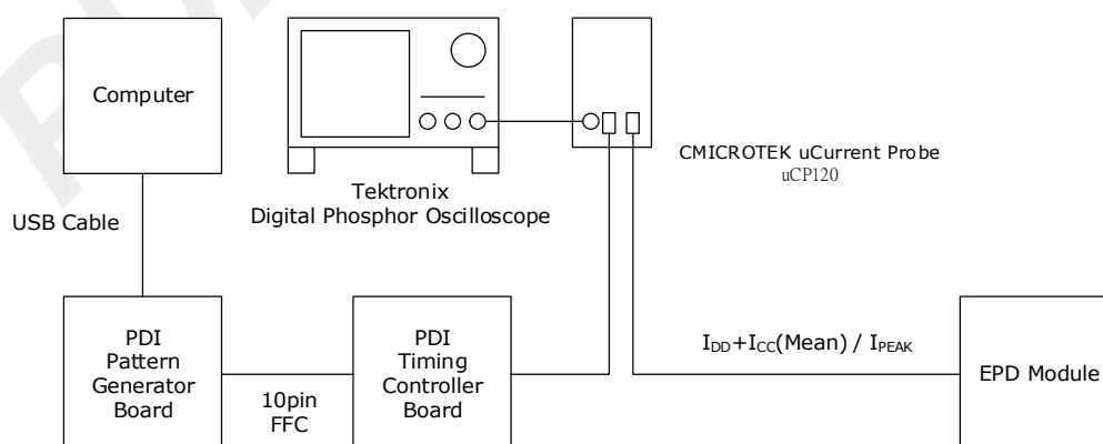
Figure 3-3 Current Measurement
