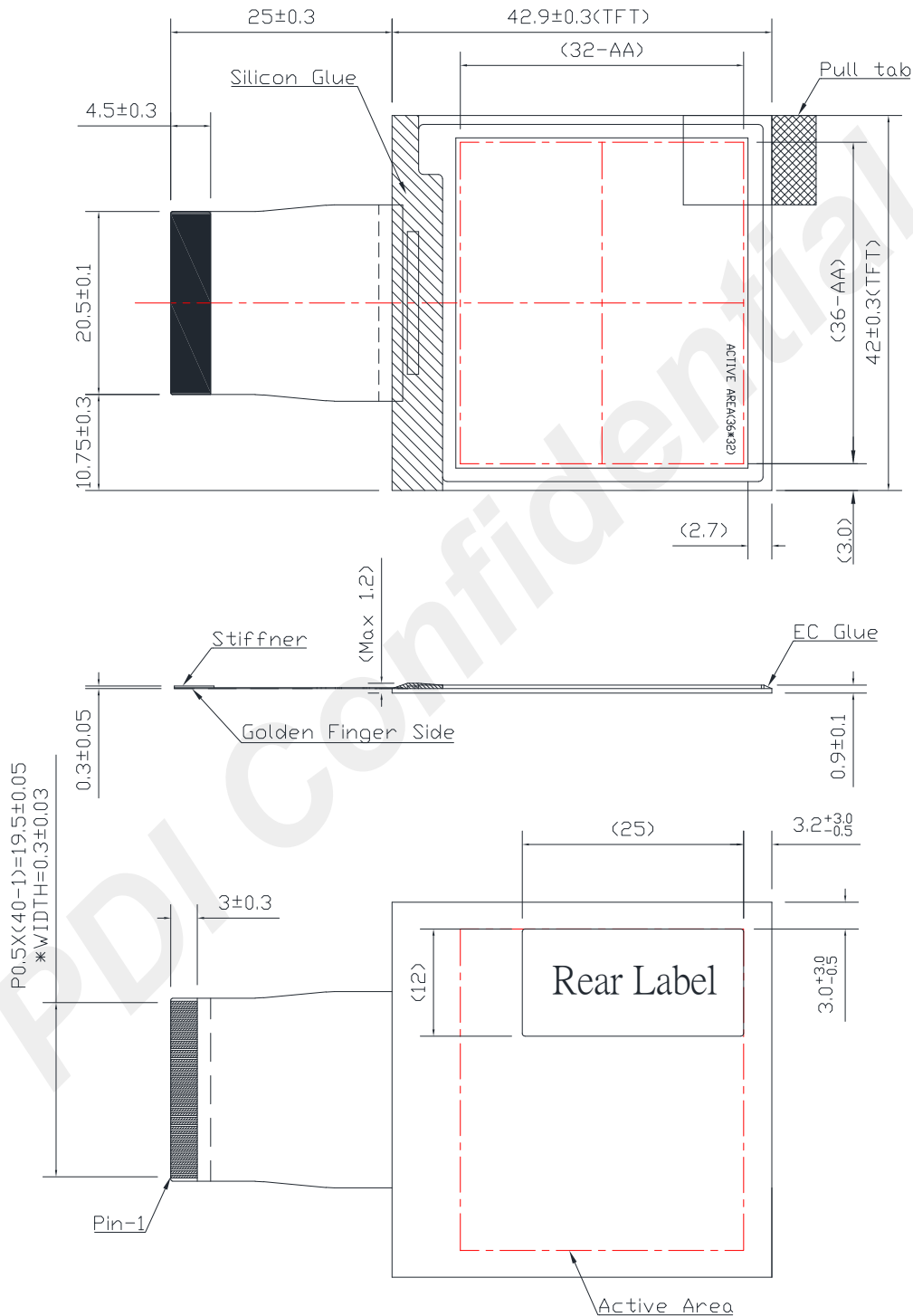
Figure 1-1 EPD Drawing
