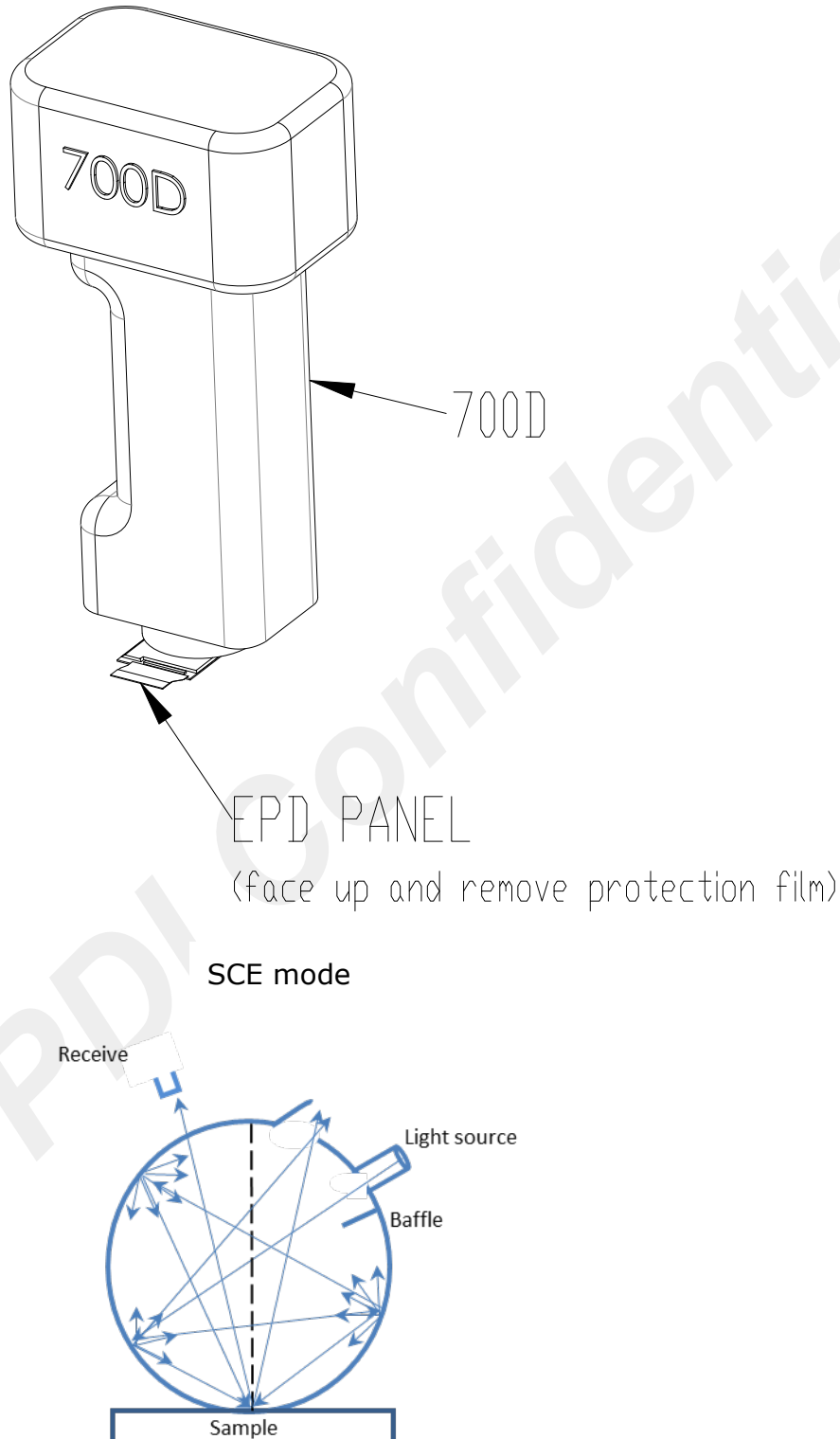
Figure 6-1 Optical measurement
