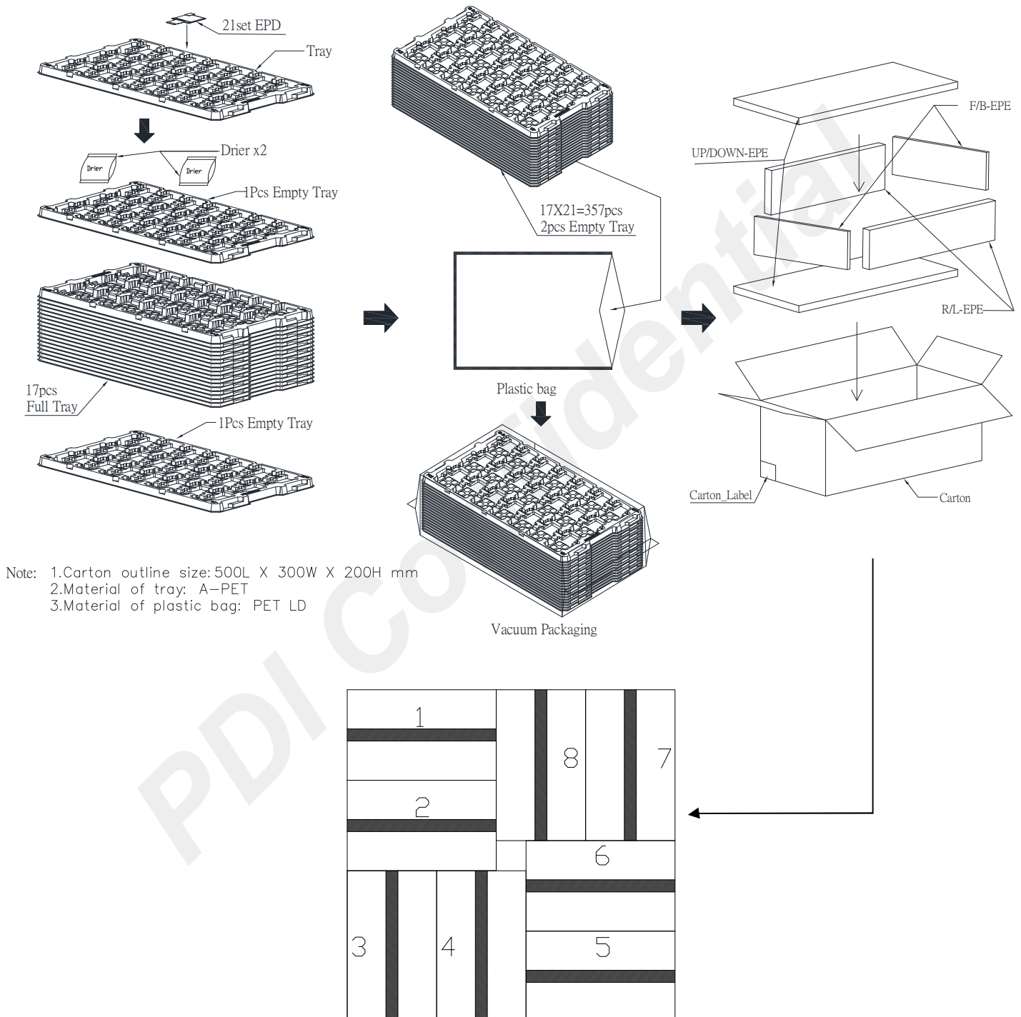
Figure 7-1 Packing Diagram
