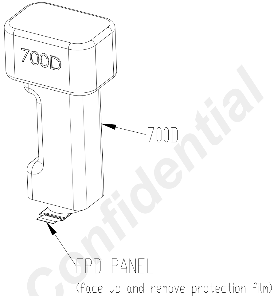
Figure 6-1 Optical measurement
