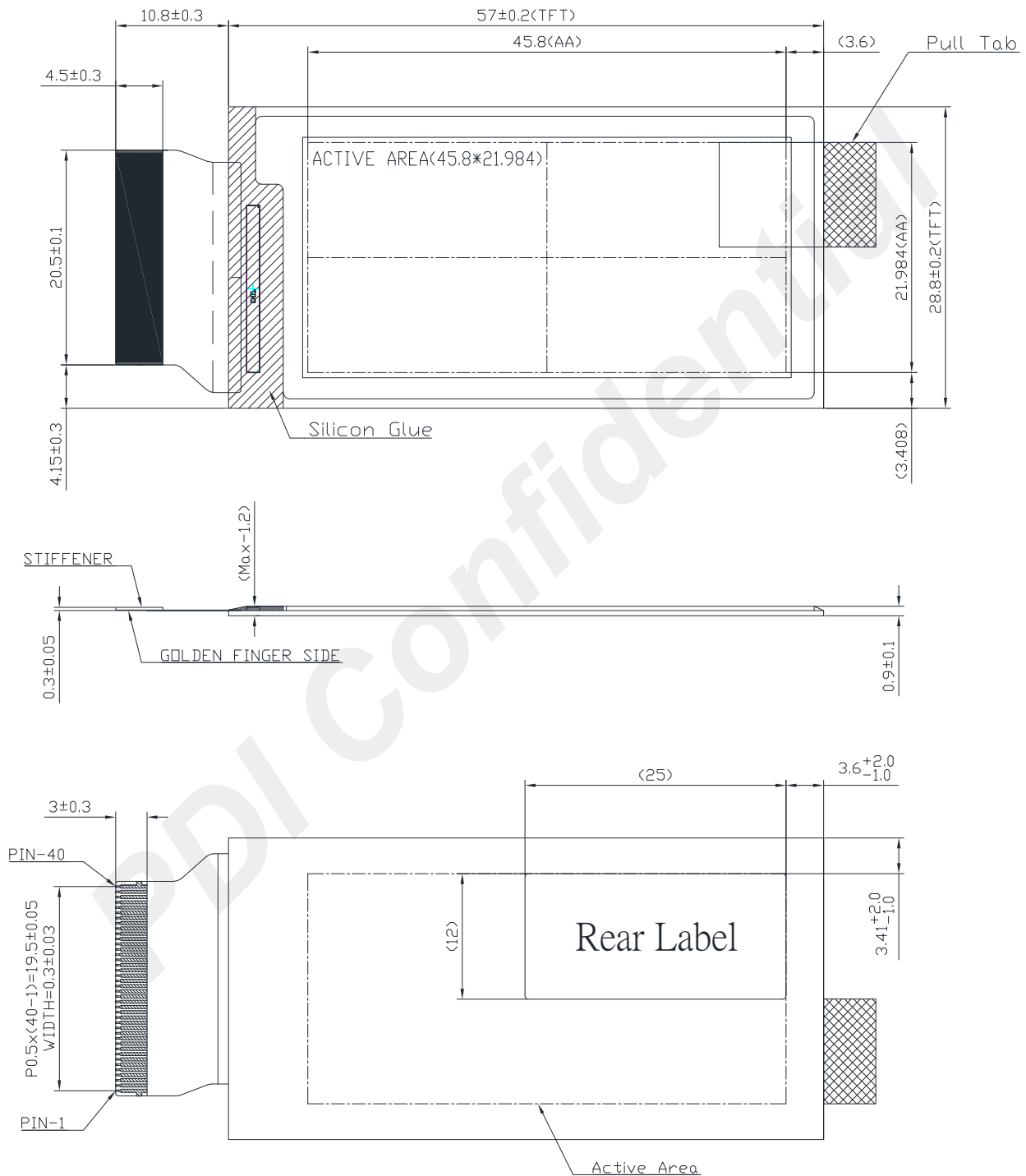
Figure 1-1 EPD Drawing
