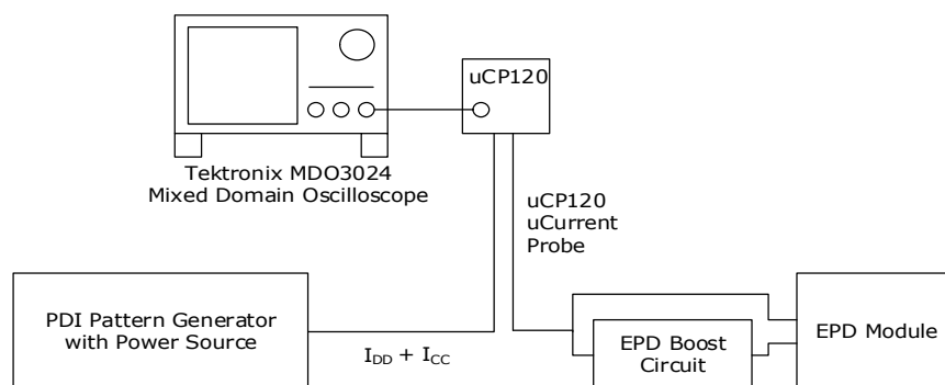
Figure 3-3 Current Measurement
