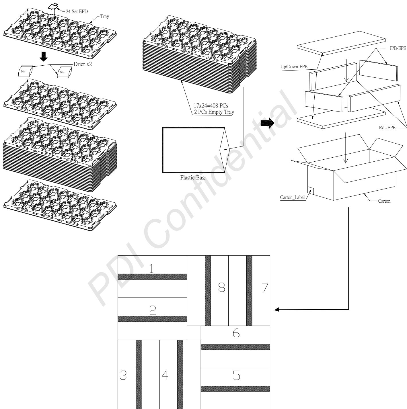
Figure 7-1 Packing Diagram
