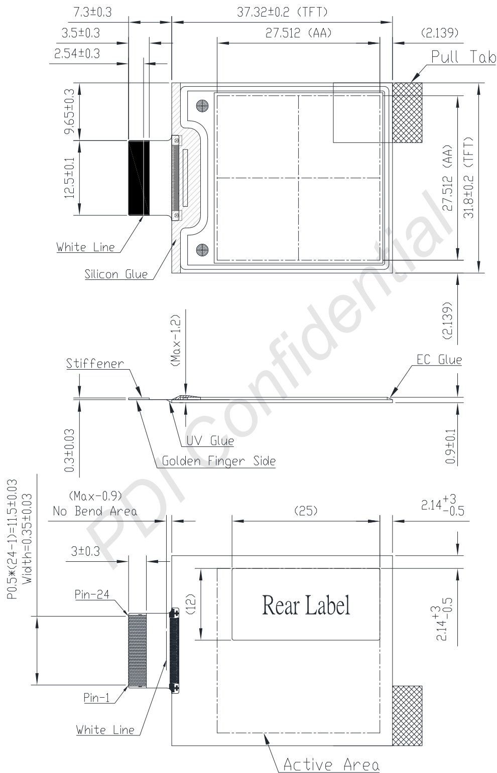
Figure 1-1 EPD Drawing
