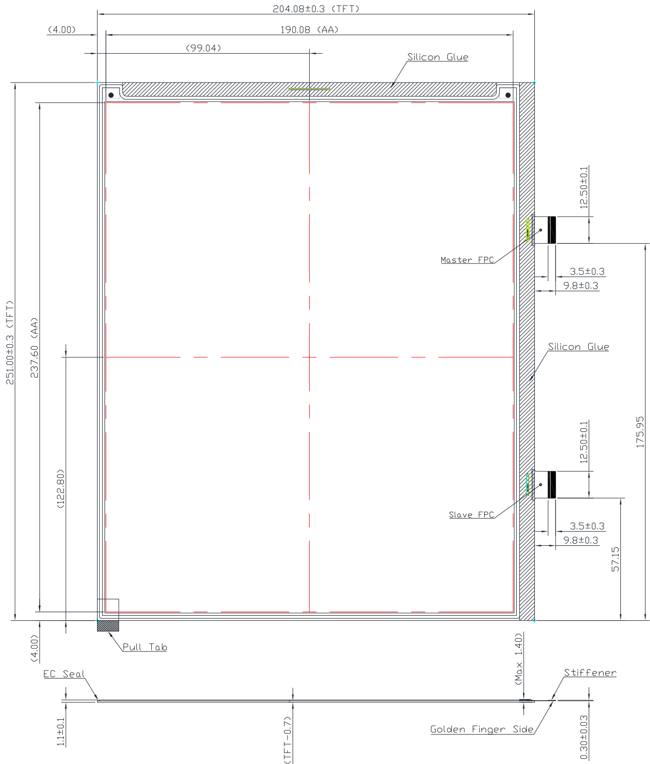
Figure 1-1 EPD Drawing
