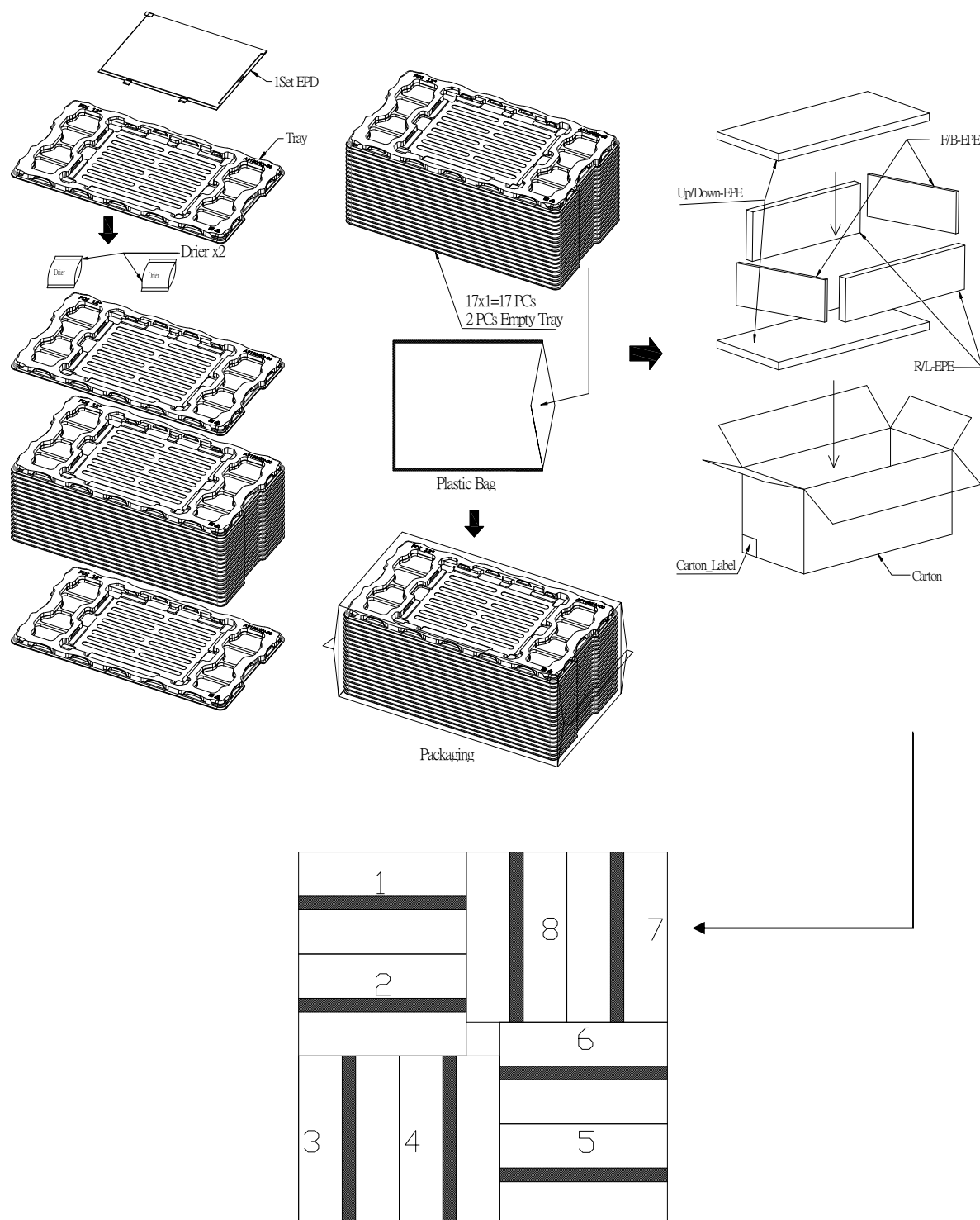
Figure 7-1 Packing Diagram
