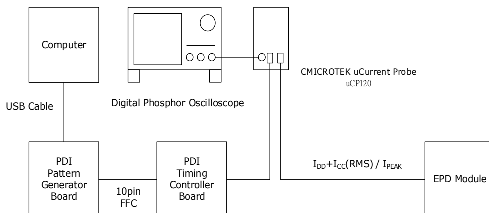
Figure 3-3 Current Measurement
