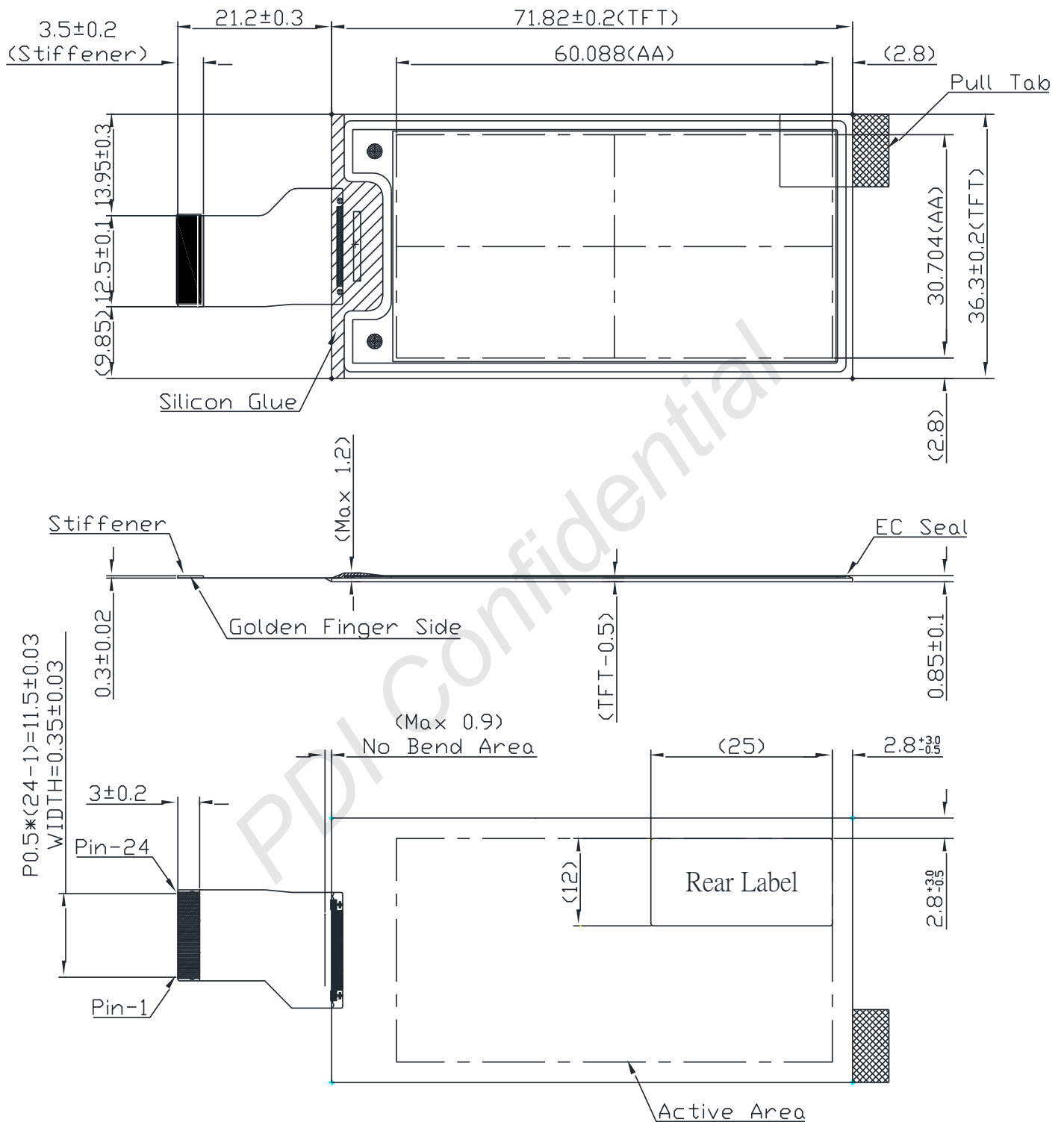
Figure 1-1 EPD Drawing
