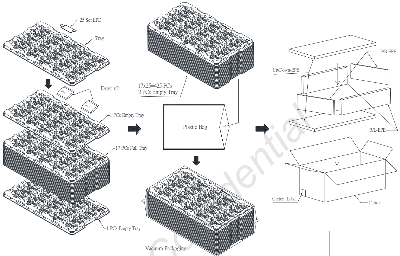
Figure 7-1 Packing Diagram
