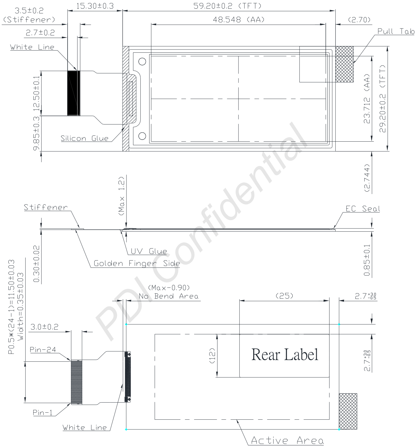
Figure 1-1 EPD Drawing
