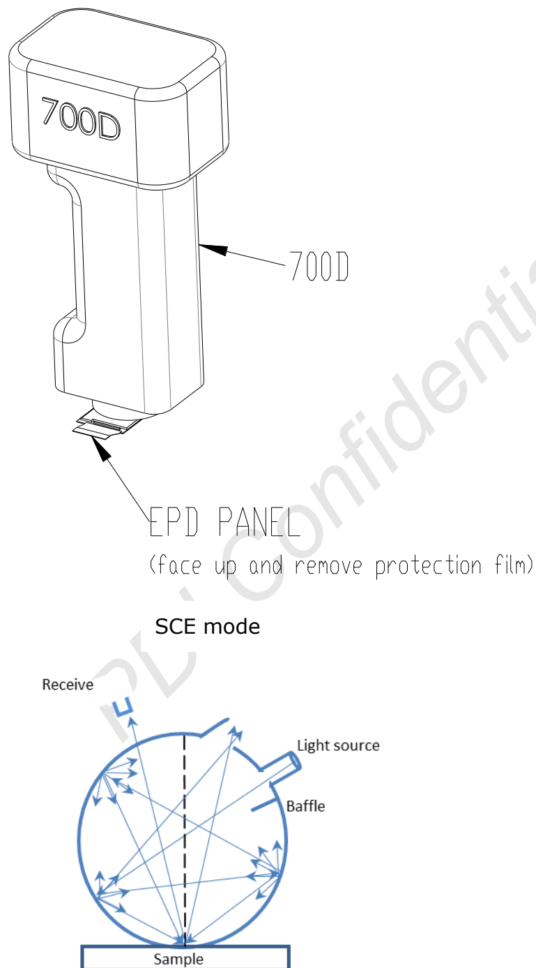
Figure 6-1 Optical measurement
