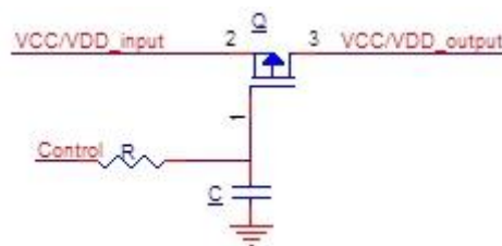
VCC/VDD soft-start
