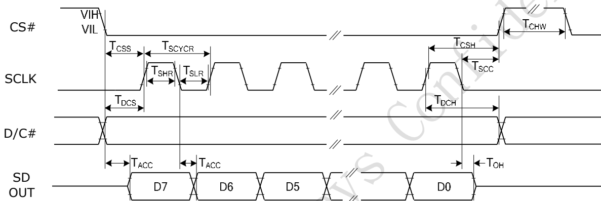
Read mode
