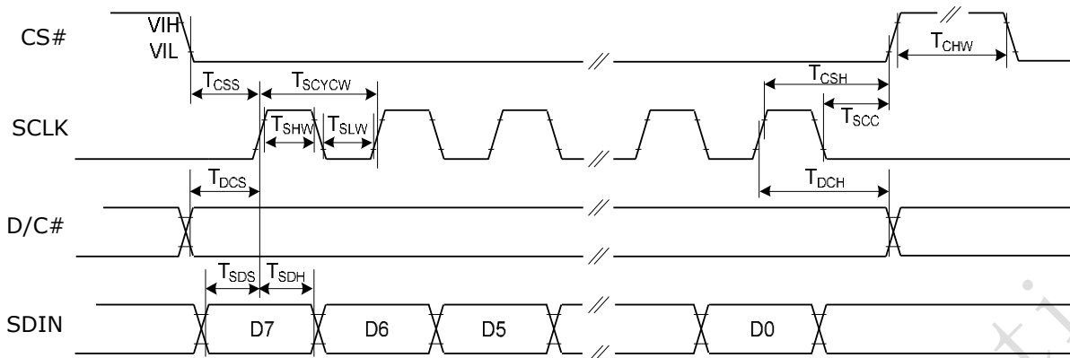
Write mode
